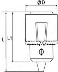
不锈钢钻夹头 Stainless Steel Drill Chucks
