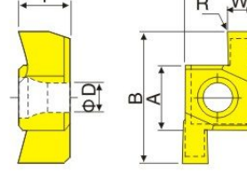
图B 双头 Fig. B Double-head
