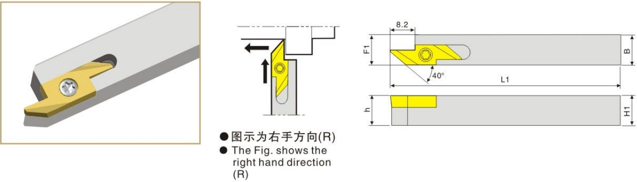
刀杆尺寸 Cutter bar dimension
